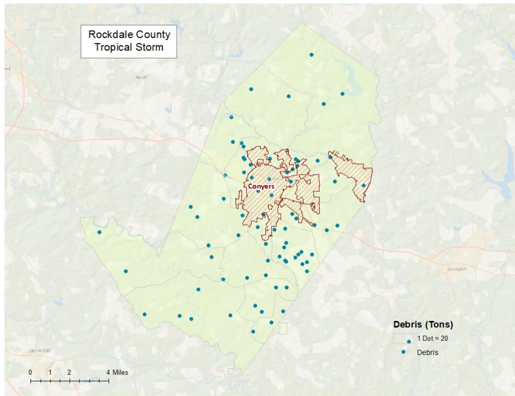
Figure 2.28 Rockdale County – Wind Related Debris in Tons (Source: HAZUS Report & POLIS Center)
