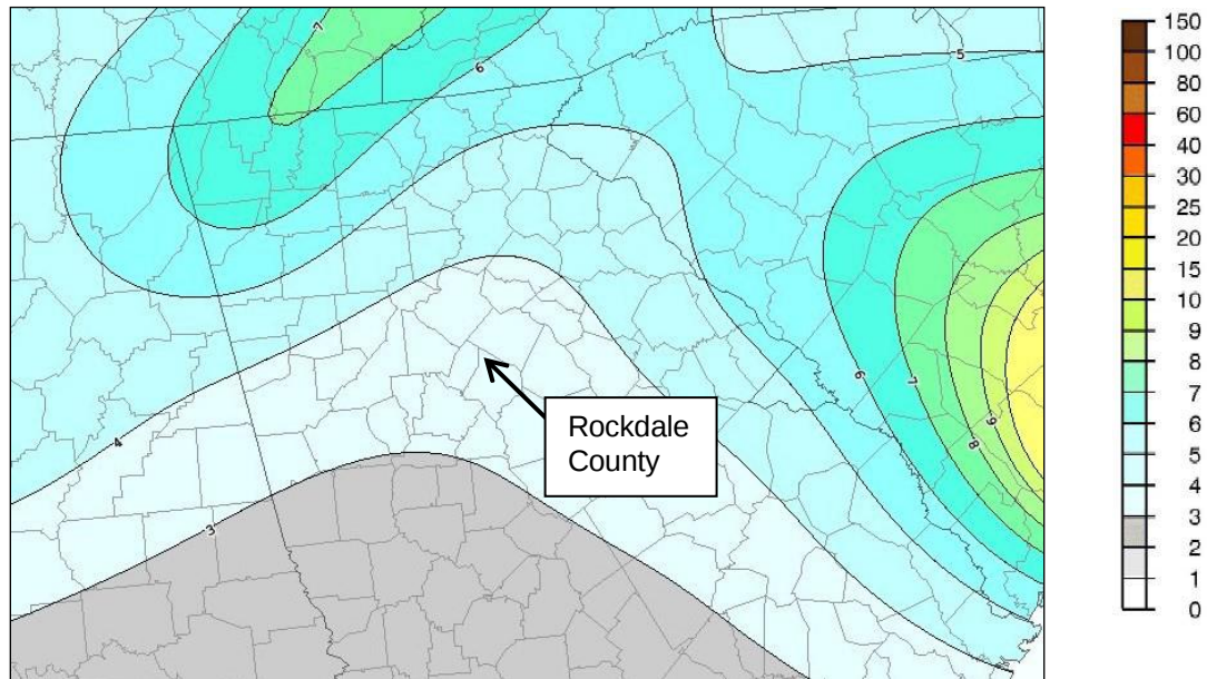
Figure 2.49 Seismic Hazard Map, showing Peak Ground Acceleration in Percent of g , with 10% exceedance in 50 years (Source: USGS, 2008)
