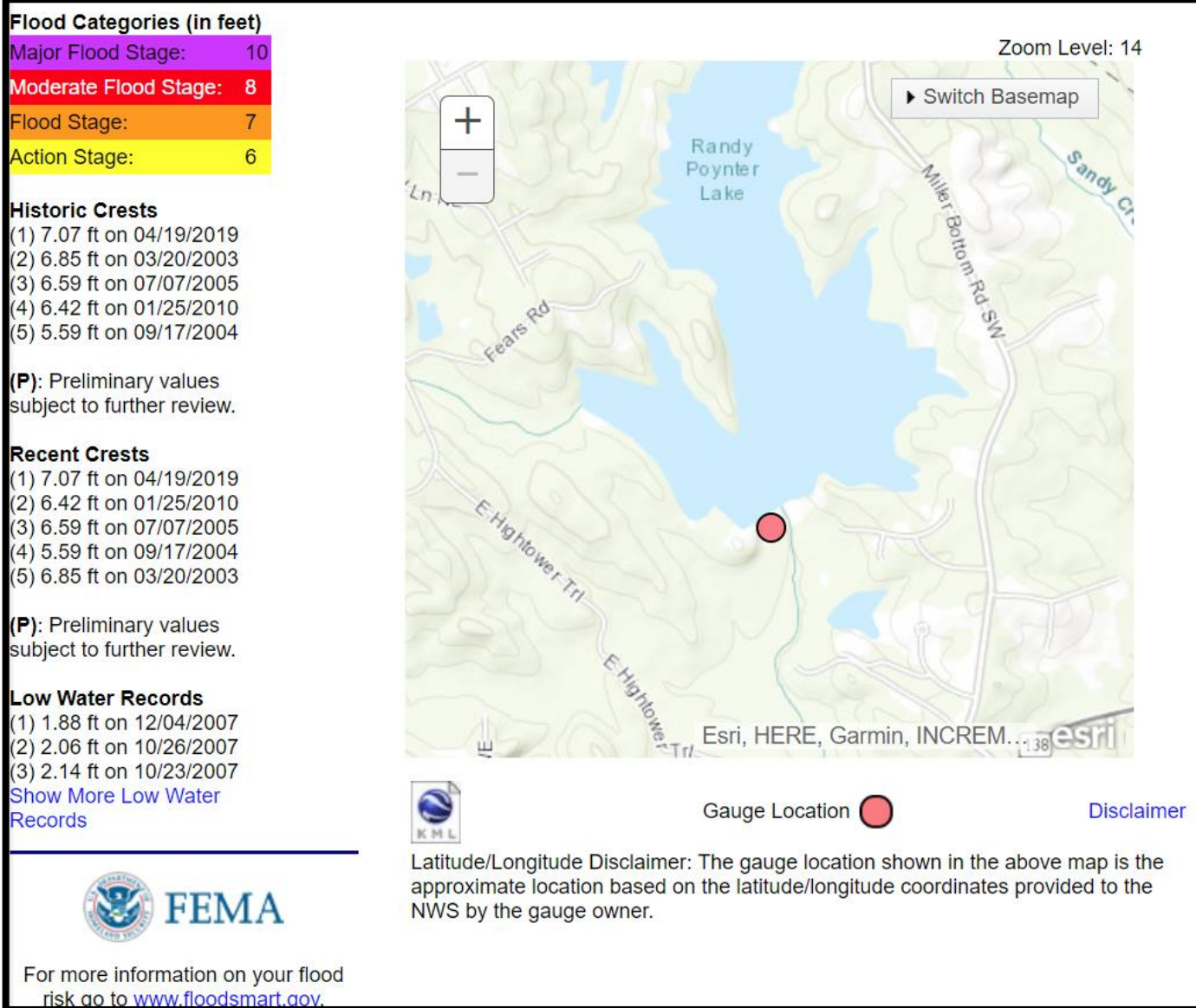
Figure 2.31 Big Haynes Creek at Jack Turner Dam near Milstead USGS 02207418 Flood Stages and Historic Crests (Source: Water.weather.gov)
