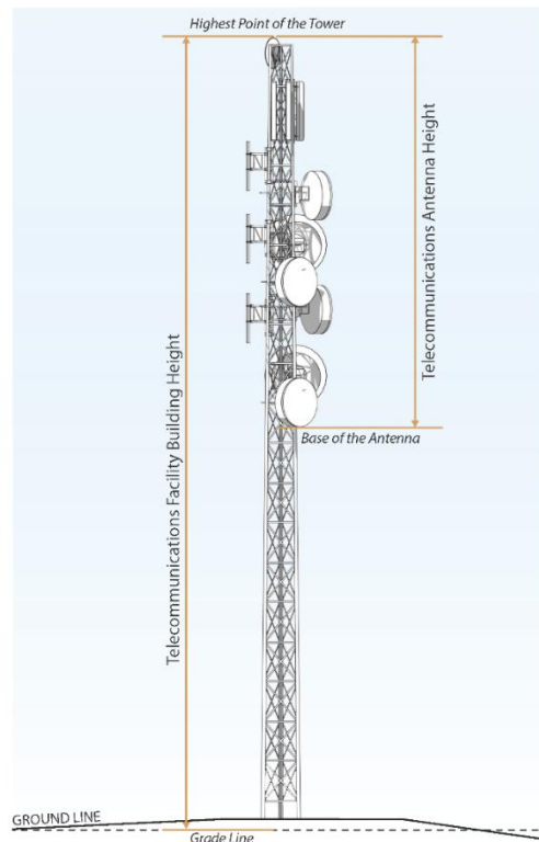
Figure 3.2.4 - Telecommunications Facility Height.
