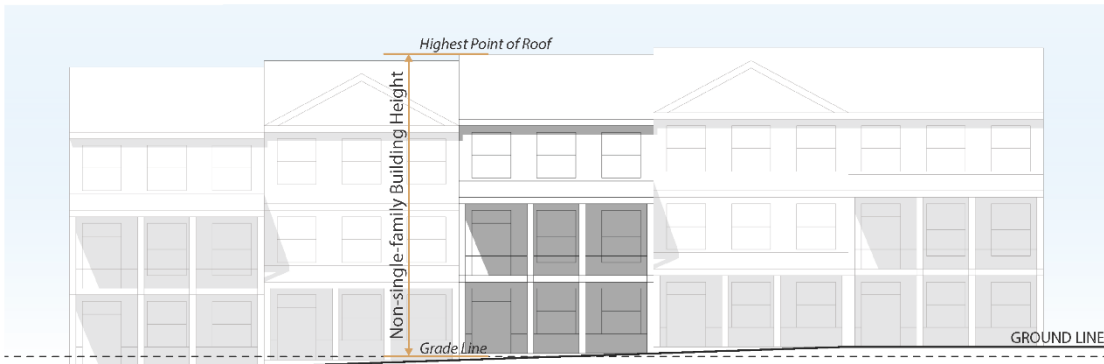
Figure 4.13.A - Measuring Non-Single-Family Residential Building Height.
