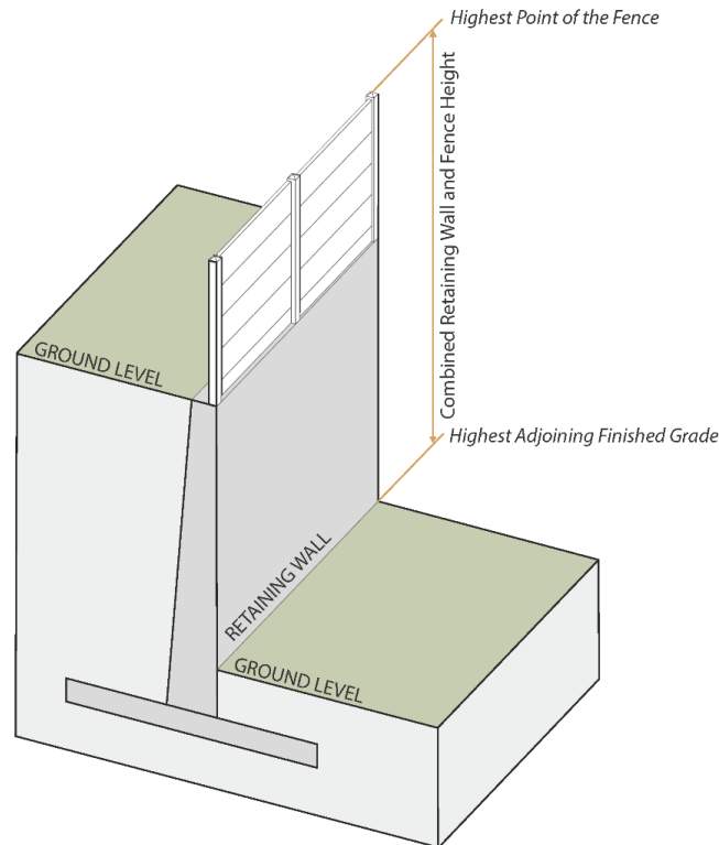
Figure 4.15.1 - Measuring Height of Fences on Retaining Walls.
